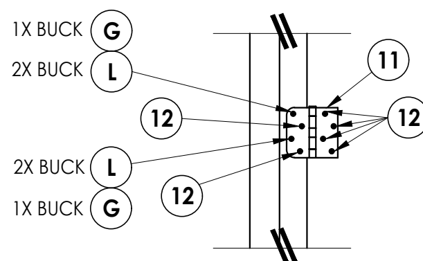
HINGE DETAIL
