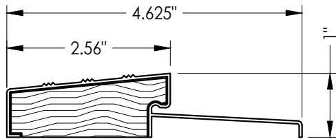
8 HEAD & SIDE Jamb (wood)
